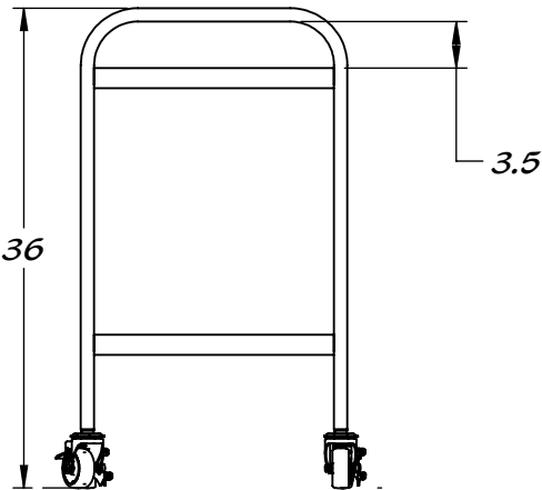
4X SWIVEL CASTERS W/BRAKE
