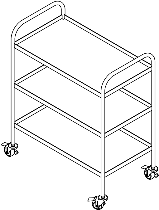
4X SWIVEL CASTERS W/BRAKE
